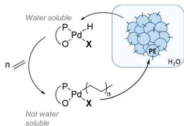
Fig. 6 Schematic of proposed mechanism showing shuttling of catalyst between the water phase and the polymer particle.
